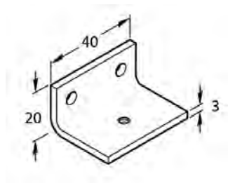
1.005 Side Fixing Bracket
