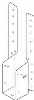
Joist Hanger (Timber to Timber)
