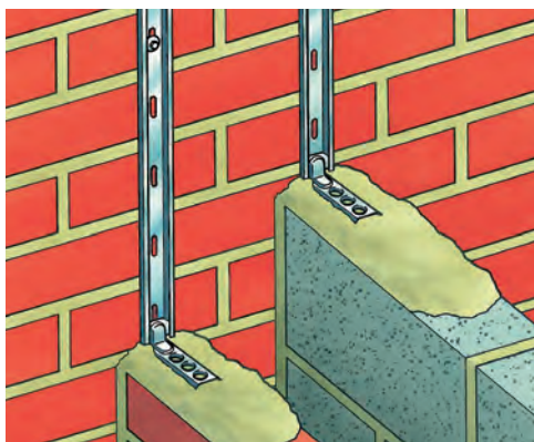
Stainless Steel Wall Starter
