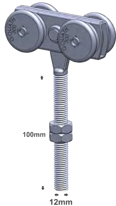
G250D Goliath G300 Double Roller (300KG) Long Stem
